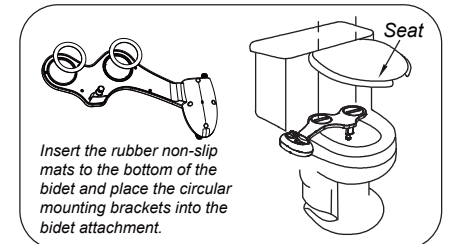
C. Install rubber non-slip mats and circular mounting brackets into bidet, and install it on toilet adjust it in suitable position
